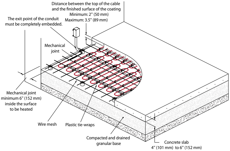
Figure 6: Concrete coating
