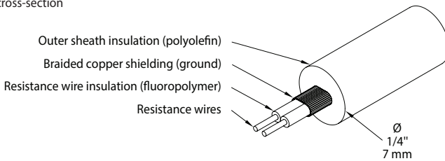
Figure 1: Cable cross-section
