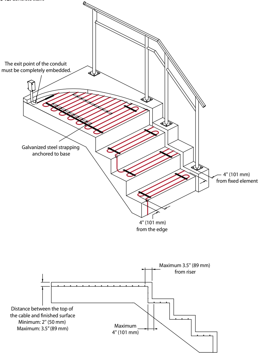
Figure 12: Concrete stairs
