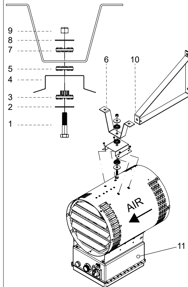
Figure 2: Mounting
