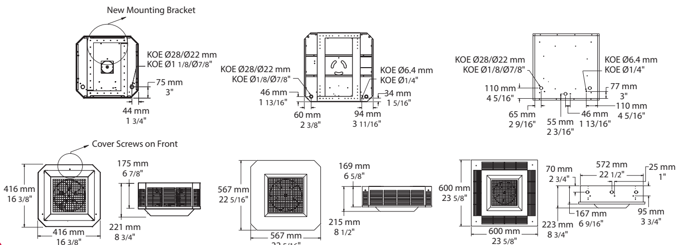
ODSA - Surface 2-5kW, 25 lbs (11.4 kg)
